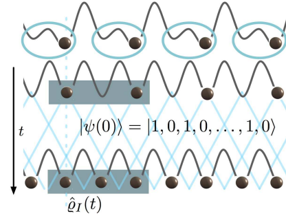
FIG. 1: Sketch of a local relaxation starting from an initial condition of bosonic atoms being present or absent, in even and odd sites of a one-dimensional Bose-Hubbard system, achieved by imposing a superlattice to an optical lattice.
