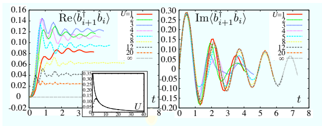
FIG. 3: Real and imaginary parts of the correlations to neighbors \langle \hat{b}_{i+1}^\dagger(t) \hat{b}_i(t) \rangle as a function of time, for different values of U . The inset shows the equilibrated value of the real part of correlations to neighbors for large t for different values of U (with a solid line proportional to 1/U as a guide to the eye).
